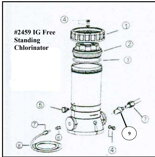
#2459 IG Free Standing Chlorinator
