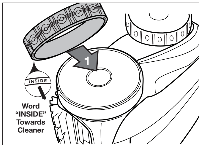
Figure 24. Tire Replacement Orientation
